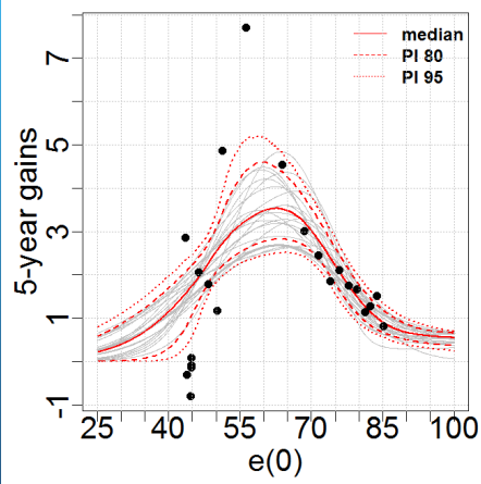
Double-logistic gain in e_0 function
