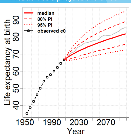
Probabilistic projections of e_0
