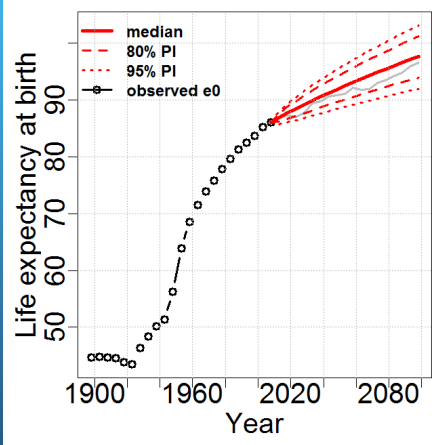
Probabilistic projections of e_0
